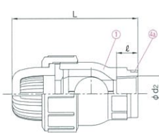
THREADED END
