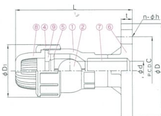
FLANGED END
