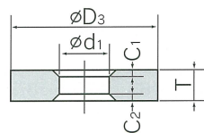
⑤ FLANGES
